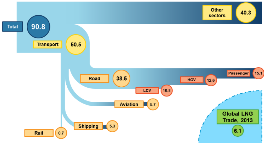
2013 Global oil demand, mbd
